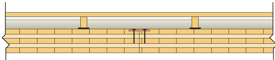
OSB wood raft with sand on top of a CLT 5 ply (131 mm)
