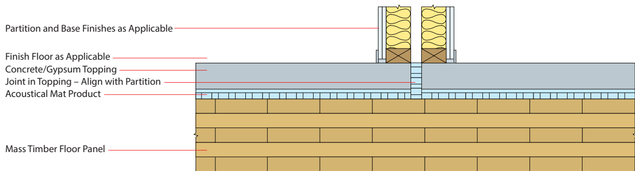
FIGURE 4: Flanking control detail at floor/wall interface
