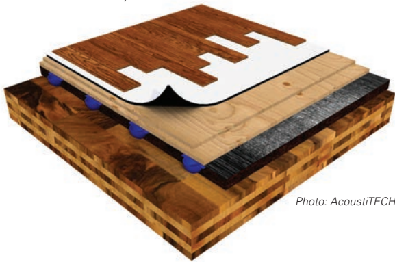
Acoustical floor underlayments
