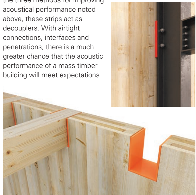
Acoustical isolation strips
