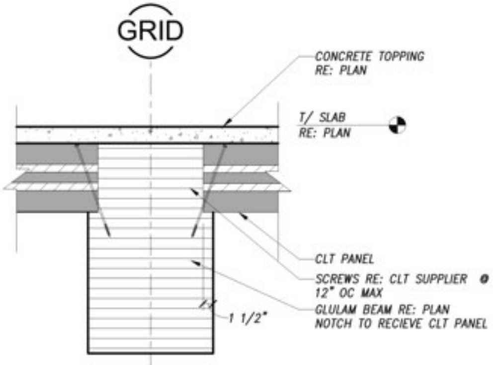
CLT TO INTERIOR BEAM CONNECTION
