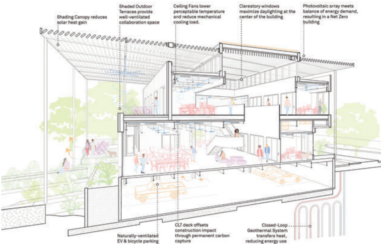
▲ Figure 2.4.5: Cross-sectional view of project, notating sustainable strategies. © Kevin Daly Architects
