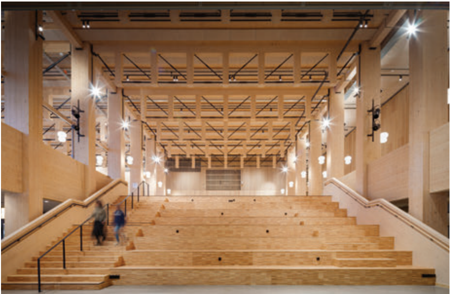
▲ Figure 2.6.11. GLT chorded trusses, augmented by steel tension rods, allow long spans over an amphitheater-style seating area on Level 1. © Martinsons | Jonas Westling
