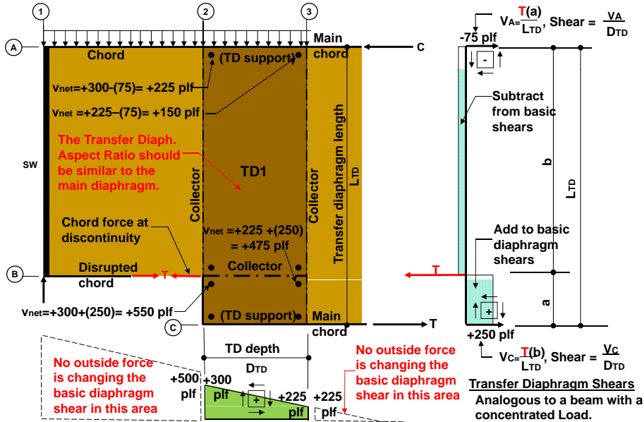
Basic Shear Diagram at transfer diaphragm
