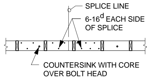
PLAN OF SILL
