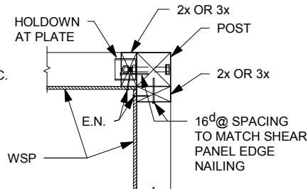
PLAN SECTION E
