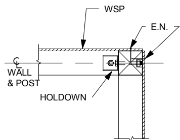
PLAN SECTION B
