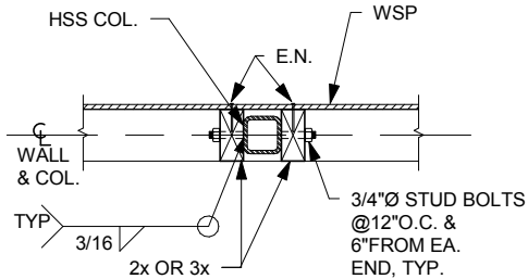
PLAN SECTION F
