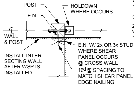
PLAN SECTION D
