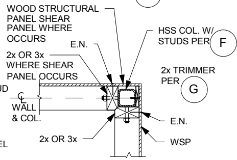
PLAN SECTION H
