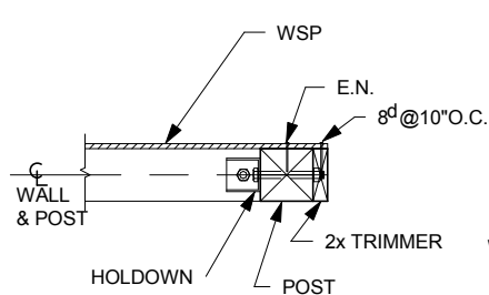
PLAN SECTION A
