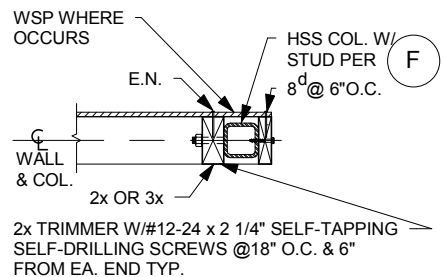
PLAN SECTION G
