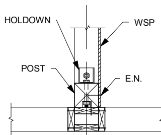
PLAN SECTION C
