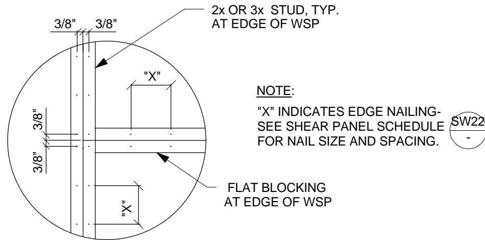
WOOD STRUCTURAL PANEL NAILING AT SPLICE (A)
