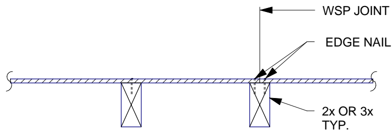
PLAN : WOOD STRUCTURAL PANEL ONE SIDE (B)
